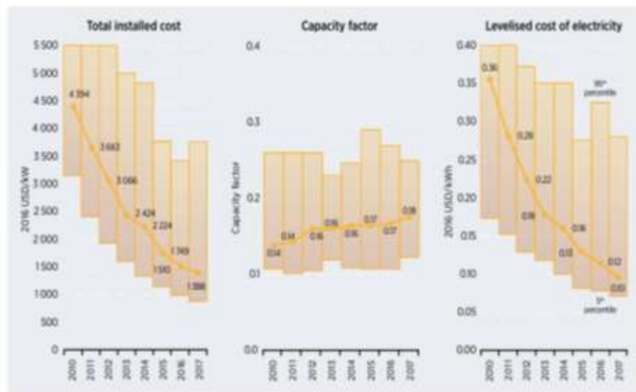
Figure 2.4 Global weighted average total installed costs, capacity factors and LCOE for solar PV, 2010-2017
